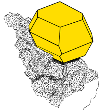
Sulfur
