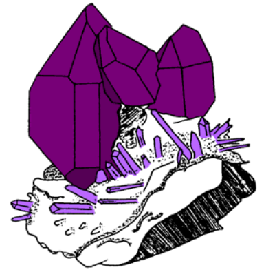
Amethyst
