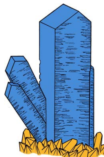
Celestine
