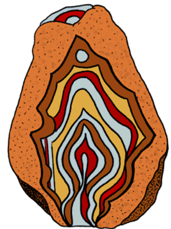
Agate
