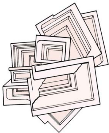
Halite
