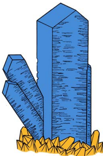
Celestine
