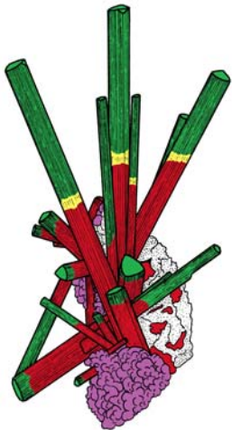
Tourmaline
