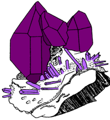
Amethyst
