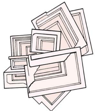
Halite
