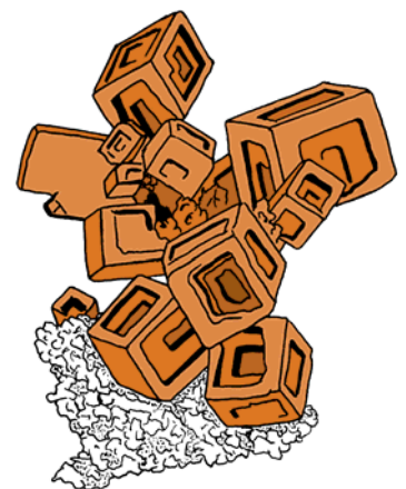
Copper
