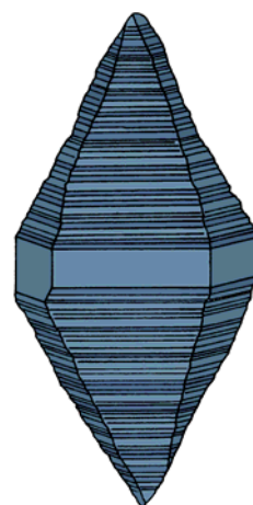
Sapphire
