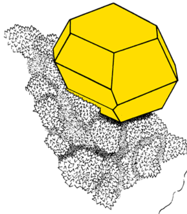
Sulfur
