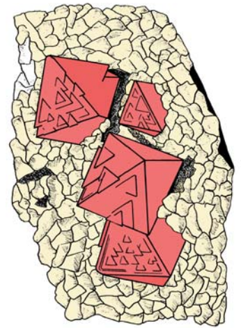
Fluorite
