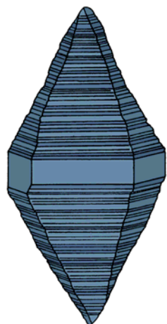
Sapphire
