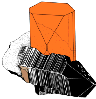
Topaz
