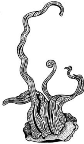
Silver
