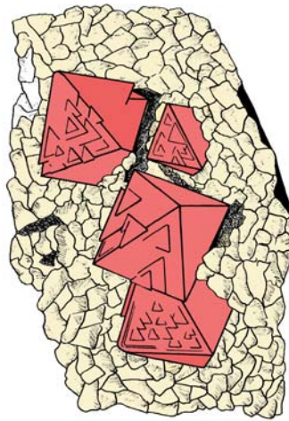
Fluorite
