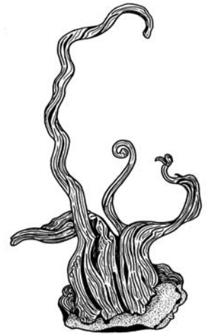
Silver
