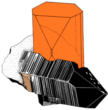
Topaz
