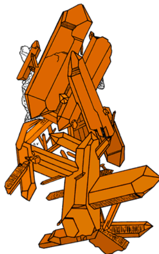
Quartz
