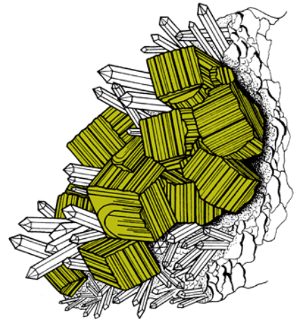
Pyrite
