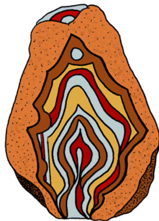
Agate
