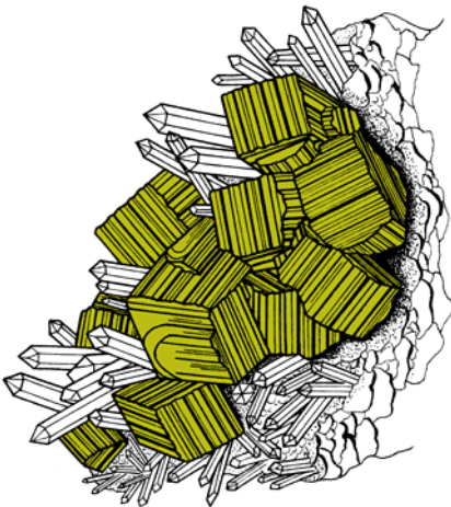
Pyrite
